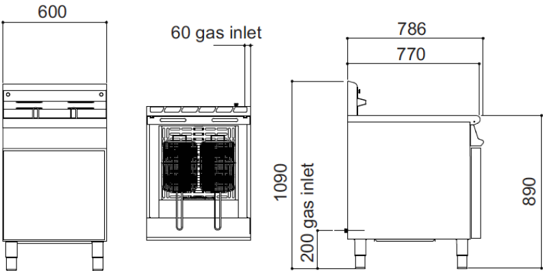
Measurements in mm Unit on castors is the same hob height
